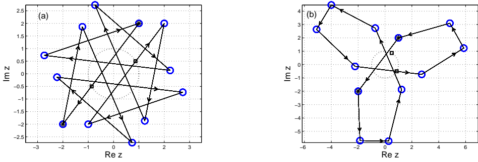
FIGURE 4. First N = 100 orbit terms of sequence \{w_n\}_{n=0}^N obtained from (2.6), for initial conditions are a = 1 + 2i and b = -2 - 2i . We compute w_0, \dots, w_N for (a) k_1 = k_2 = 12 , z_1 = e^{2\pi i \frac{1}{12}} , z_2 = e^{2\pi i \frac{7}{12}} ; (b) k_1 = 2k_2 = 12 , z_1 = e^{2\pi i \frac{1}{6}} , z_2 = e^{2\pi i \frac{11}{12}} . Arrows indicate the direction of the orbit from one term to the next. The dotted line is the unit circle.
