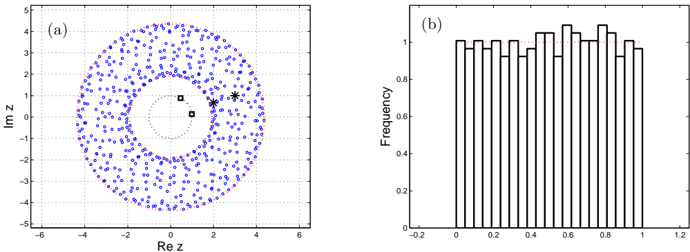
FIGURE 5. (a) First N = 1001 terms of \{w_n\}_{n=0}^\infty given by (2.6) when z_1 = e^{2\pi i \frac{4}{23}} , z_2 = e^{2\pi i \frac{2}{89}} (squares) and a = 2 + 2/3i , b = 3 + i (stars). The solid line represents the unit circle. Boundaries of annulus U(0, ||A| - |B||, |A| + |B|) from (4.20) are also represented; (b) Histogram of arguments \text{Arg}(w_n) , n = 0, \dots, 1000 .
