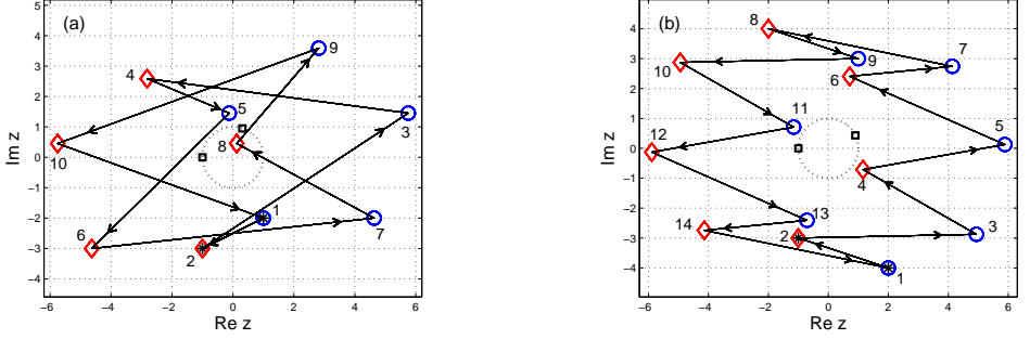
FIGURE 2. First N = 100 orbit terms of \{w_n\}_{n=0}^N obtained from (2.6), for z_2 = -1 and (a) k = 5 (odd), z_1 = e^{2\pi i \frac{1}{5}} and a = 2 - 4i , b = -1 - 3i ; (b) k = 14 (even), z_1 = e^{2\pi i \frac{1}{14}} and a = 1 - 2i , b = -1 - 3i . Arrows indicate the direction of the orbit visiting w_0, w_1 (star), w_2, \dots, w_N . The sets W_0 and W_1 defined in (3.10) and (3.13) are represented by circles and diamonds respectively. The dotted line represents the unit circle.
