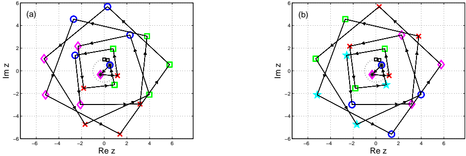
FIGURE 3. First N = 100 orbit terms of sequence \{w_n\}_{n=0}^N obtained from (2.6), for k_1 = 4, k_2 = 5 . We compute w_0, \dots, w_N for z_1 = e^{2\pi i \frac{1}{5}}, z_2 = e^{2\pi i \frac{1}{4}} and initial conditions a = (1 + i)/2, b = -(1 + i)/3 . The orbits are partitioned into (a) four regular pentagons; (b) five squares; Arrows indicate the direction of the orbit from one term to the next. The dotted line is the unit circle.
