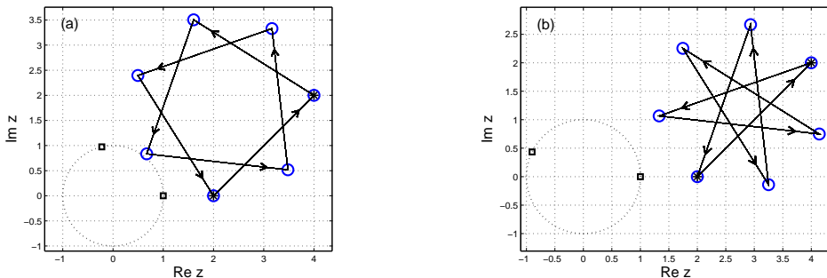
FIGURE 1. First N = 100 orbit terms of sequence \{w_n\}_{n=0}^N obtained from (2.6), for z_2 = 1 and (a) k = 7 , z_1 = e^{2\pi i \frac{2}{7}} ; (b) k = 7 , z_1 = e^{2\pi i \frac{3}{7}} ; when a = 2 and b = 4 + 2i . Arrows indicate the direction of the orbit visiting w_0, w_1 (star), w_2, \dots, w_N (circle). The dotted line represents the unit circle.
