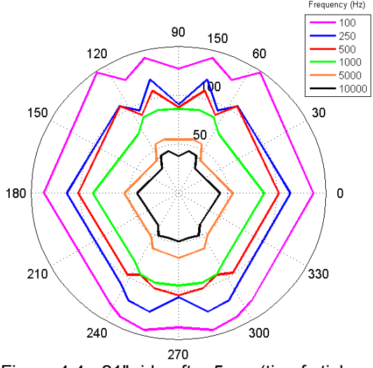
Figure 4.4 - 21" ride after 5 ms (tip of stick on centre of bow)
