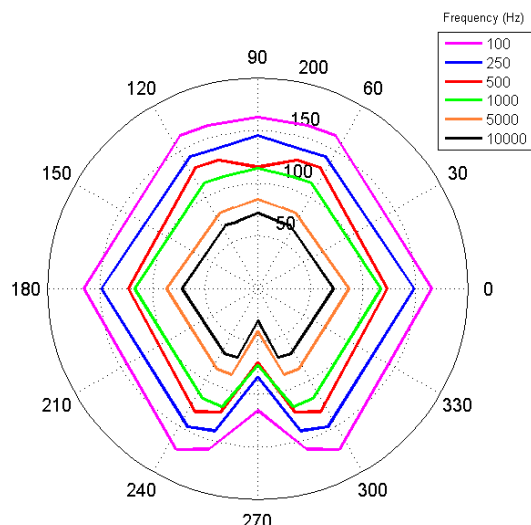
Figure 4.6 - 14" hi-hats after 5 ms (open)
